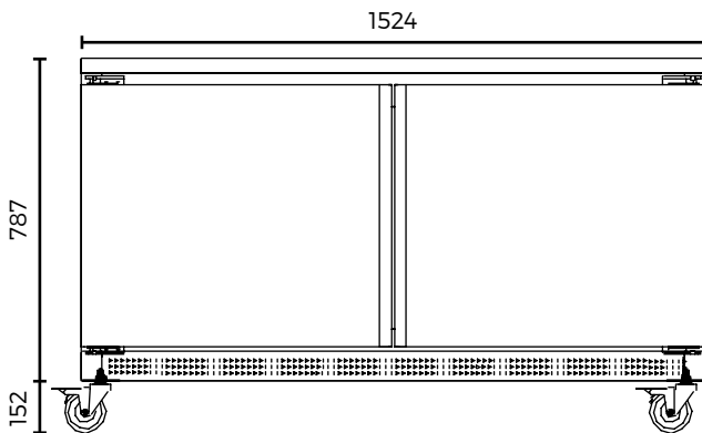
AUTR-60 / AUTF-60
