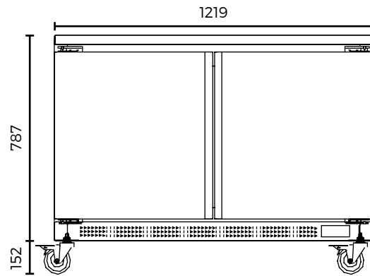
AUTR-48 / AUTF-48
