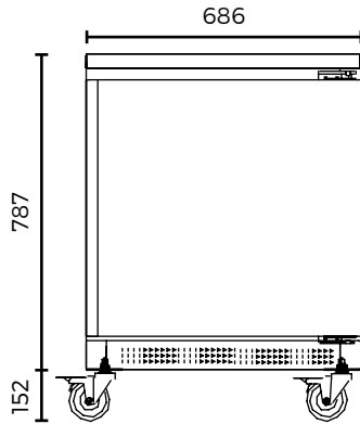
AUTR-27 / AUTF-27
