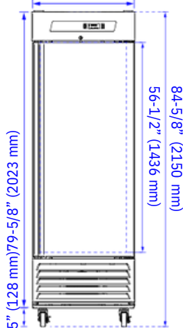
27-1/2" (700 mm)
